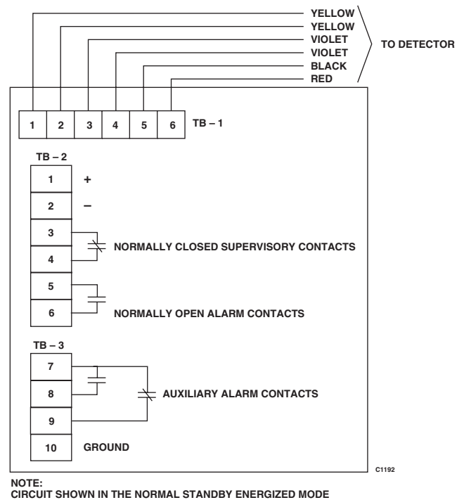
Figure 3—Wiring Terminals
