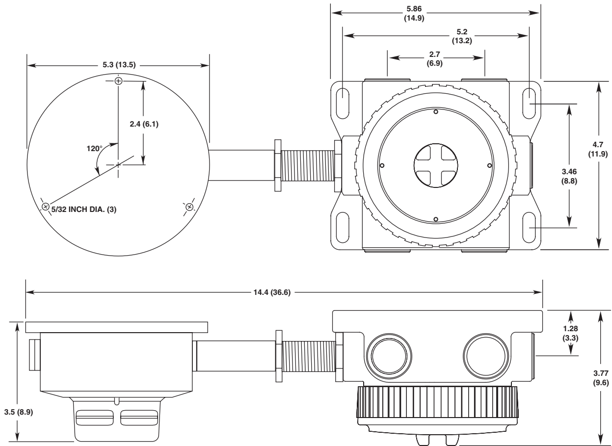
Figure 2—U5005 Dimensions in Inches (centimeters)
