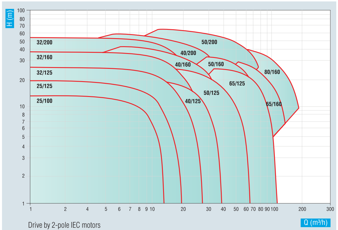
Performance curves for submersible centrifugal pumps with nominal speed 2900 1/min.
