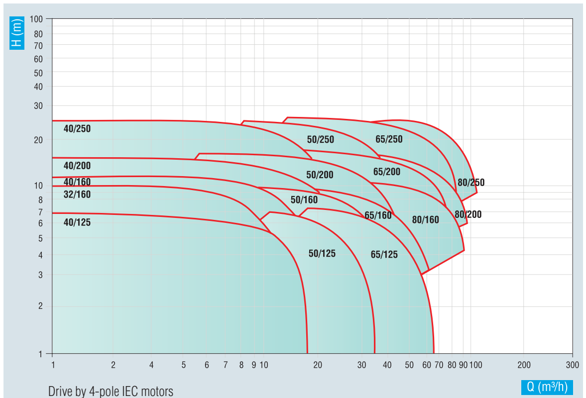
Performance curves for submersible centrifugal pumps with nominal speed 1450 1/min.
